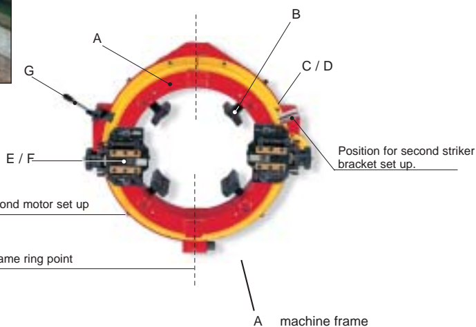
Our spring loaded dancer tool boxes follow the contour of the pipe to give you an accurate weld prep.
